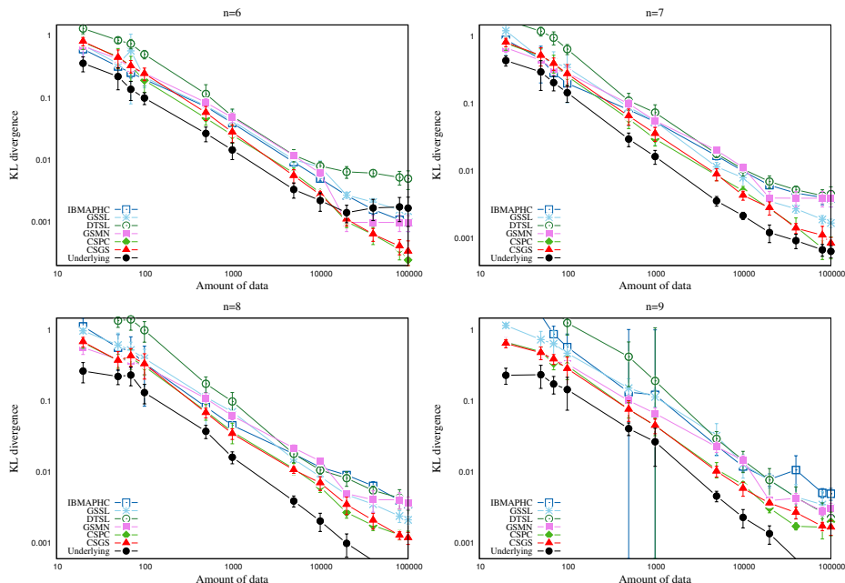
Fig. 1. KL divergences over increasing amounts of data for structures learned by: CSGS, CSPC, IBCMAP-HC, GSMN, GSSL, and DTSL. For comparison reasons, the KL divergence of the underlying structure is shown. Every point represents the average and standard deviation over ten datasets with a fixed size.
